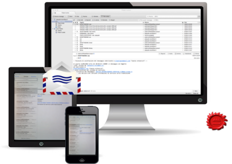
Fig 2. Interfaccia Client
